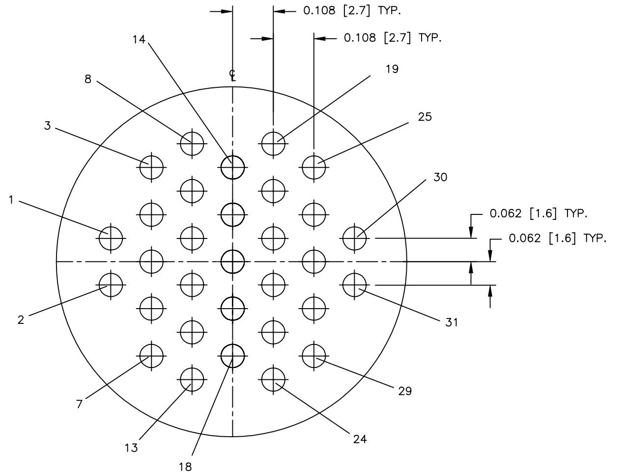
31-#20 PC TAIL DIA. 0.0395 ±0.001 REF. PANEL PIN
