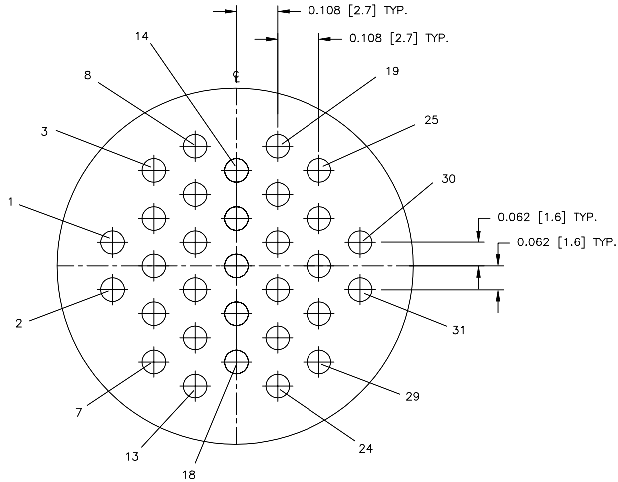
31-#20 PC TAIL DIA. 0.0395 ±0.001 REF. PANEL SOCKET
