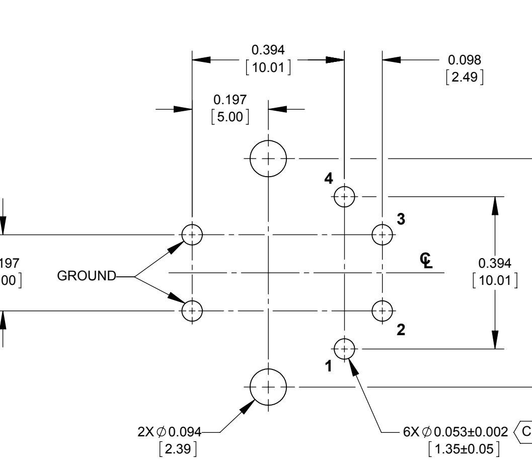
RECOMMENDED PC BOARD LAYOUT COMPONENT SIDE
